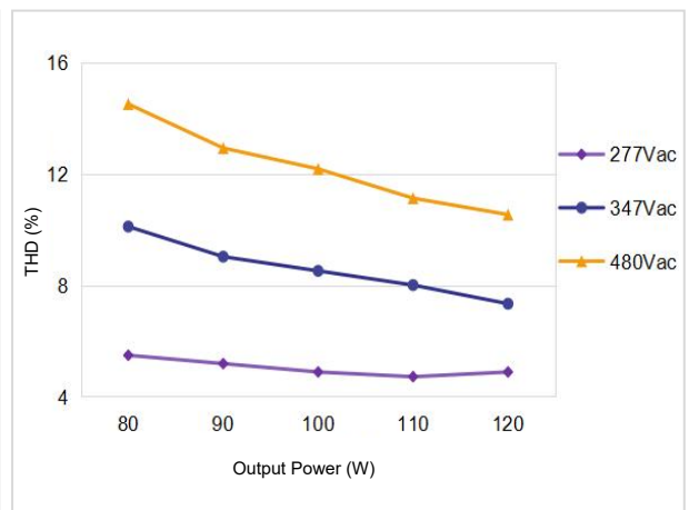
THD
