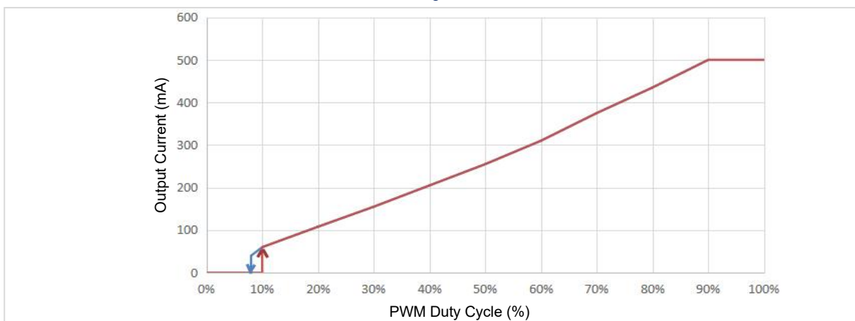
Dimming Curve
