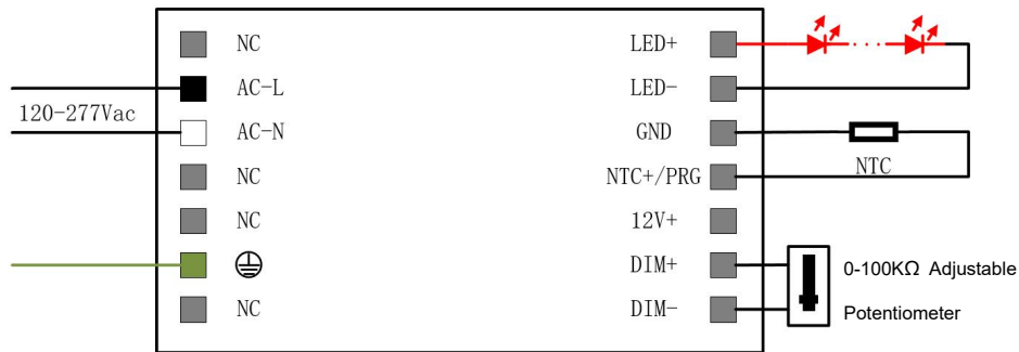
Wiring diagram of Rx dimmer
