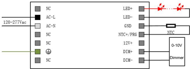
Wiring diagram of 0-10V dimmer
