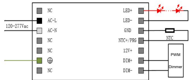
Wiring diagram of PWM dimmer
