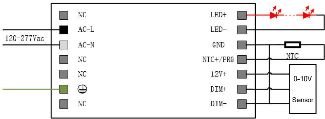
Wiring diagram of 0-10V sensor
