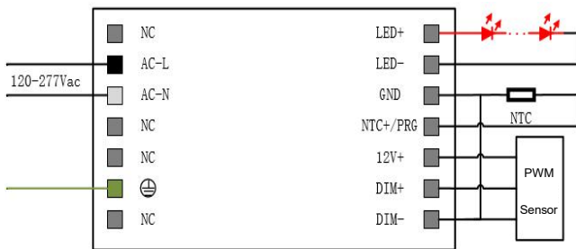
Wiring diagram of PWM sensor
