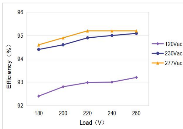
Power Curve
