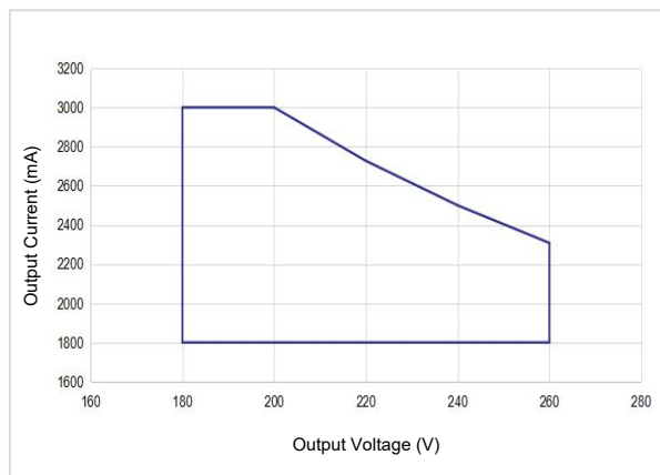
Power Curve
