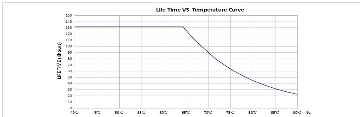
Lifetime Curve
