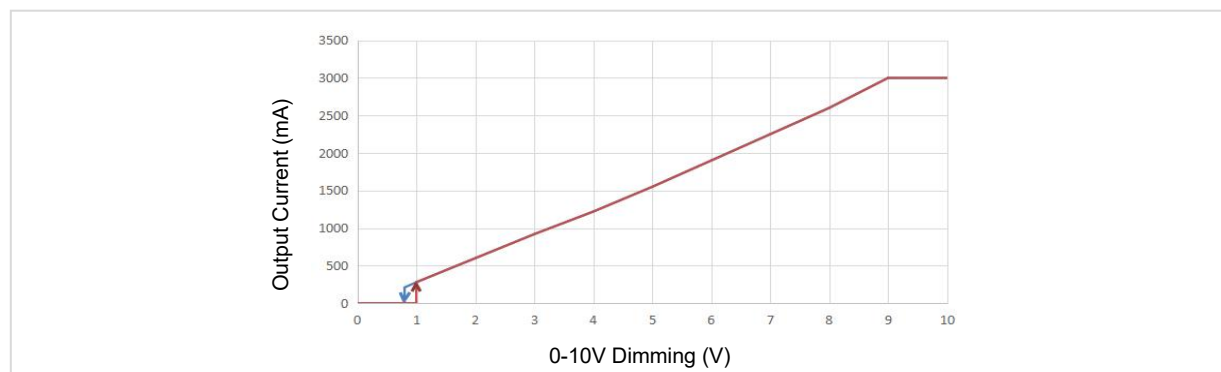
Dimming Curve
