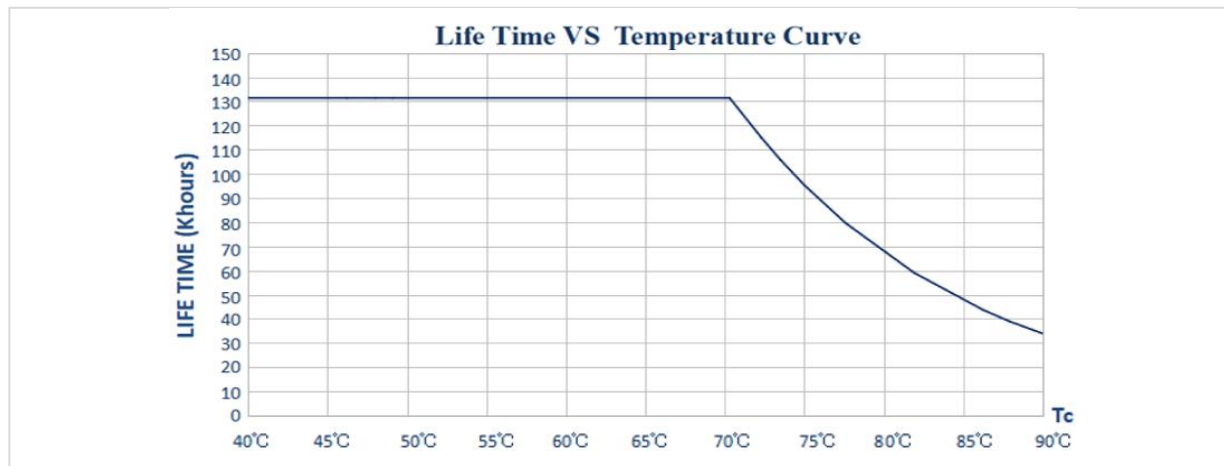
Lifetime Curve
