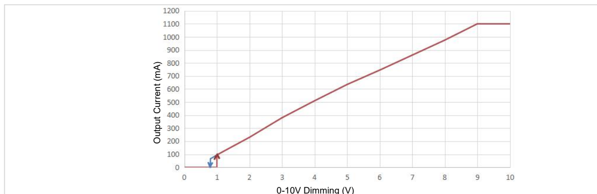
Dimming Curve
