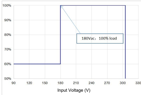
Power Curve (300-450mA @100~180Vac)
