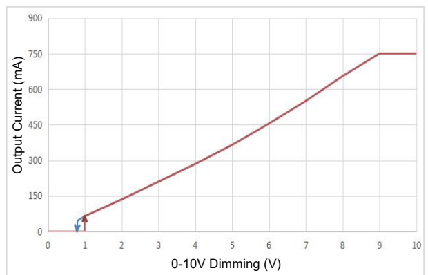
Dimming Curve
