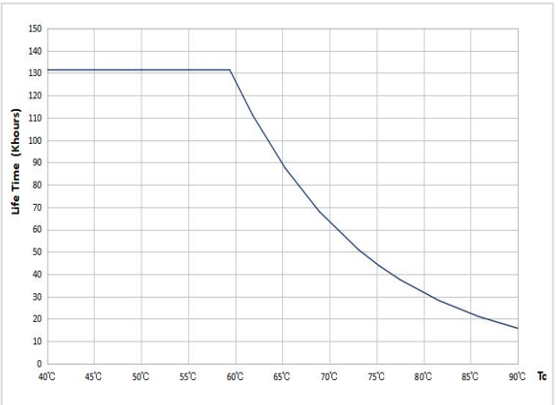
Lifetime Curve
