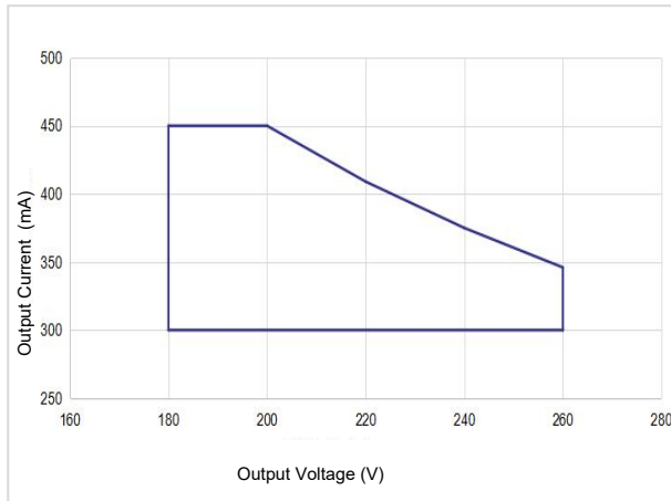
Power Curve (300-450mA @100~180Vac)
