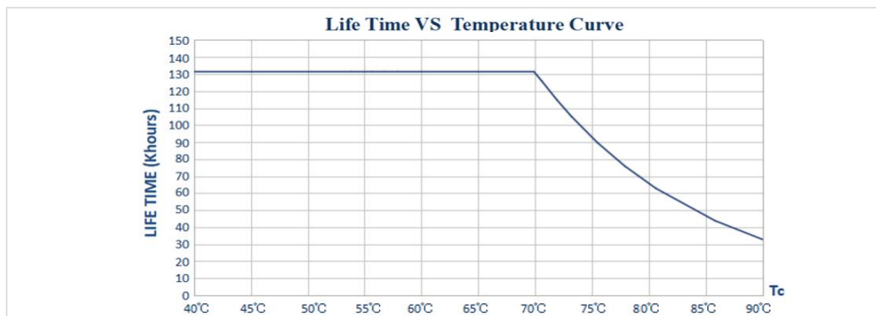
Lifetime Curve
