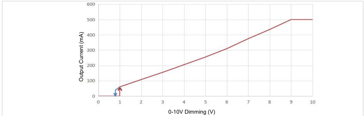
Dimming Curve
