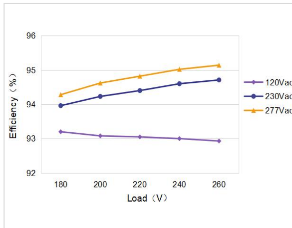
Efficiency Curve
