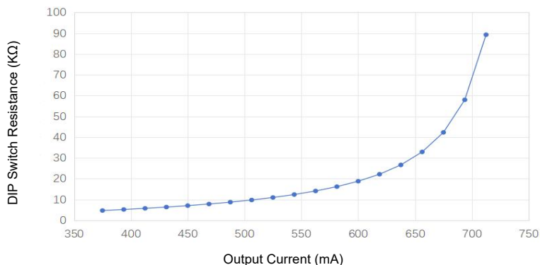
Curve of DIP Switch Resistance and Output Current
