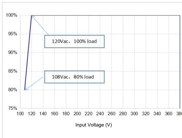
Power Derating
