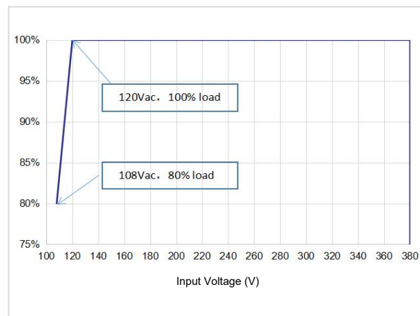
Power Derating
