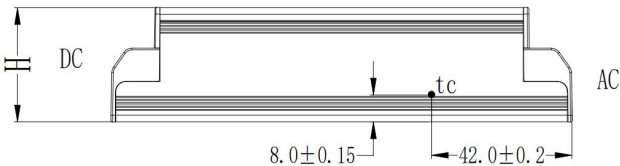
Tc point is on the side of LED driver
