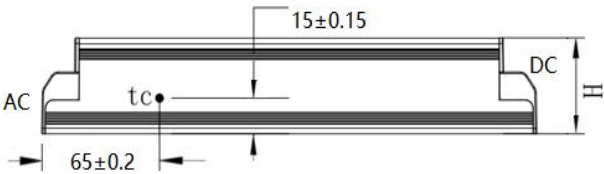
Tc point is on the side of LED driver
