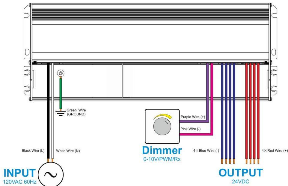
Wiring diagram of 3-in-1 dimming
