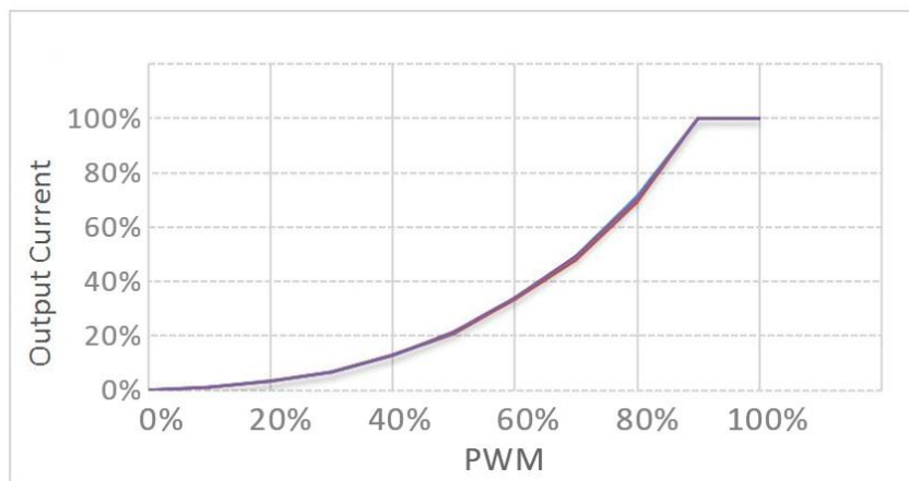
PWM dimming
