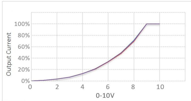
0-10V dimming
