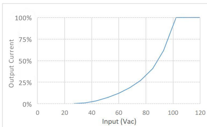
Triac dimming
