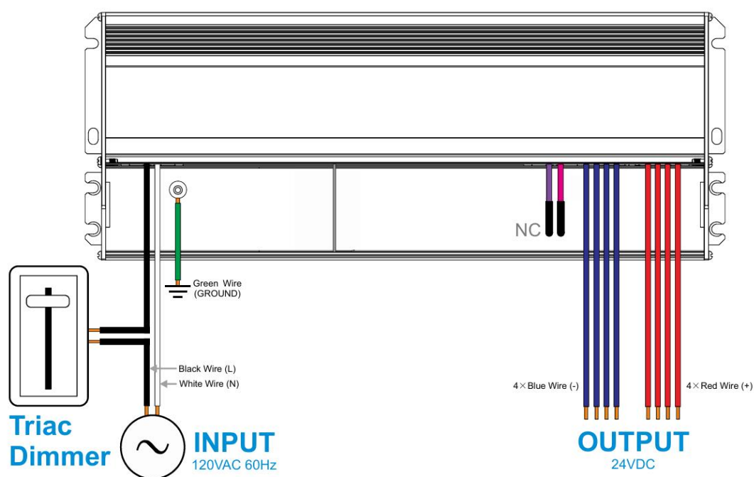
Wiring diagram of Triac dimming
