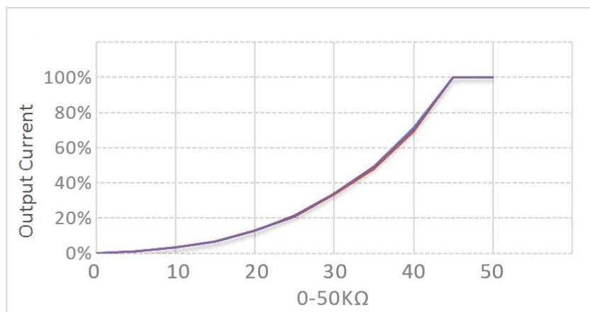
Rx dimming
