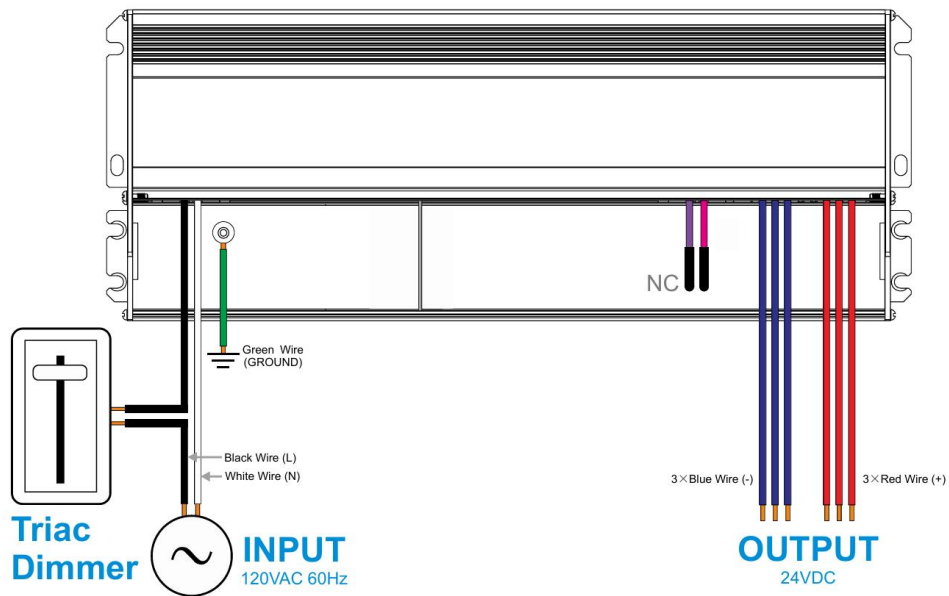
Wiring diagram of Triac dimming
