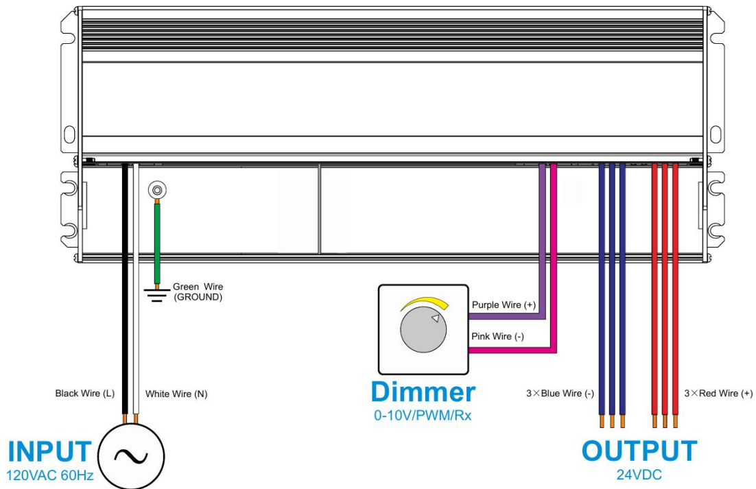
Wiring diagram of 3-in-1 dimming
