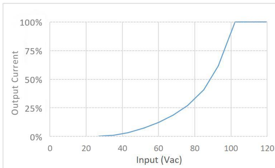
Triac dimming
