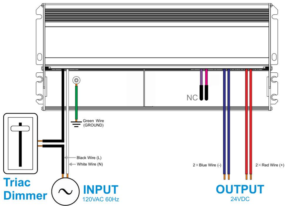
Wiring diagram of Triac dimming
