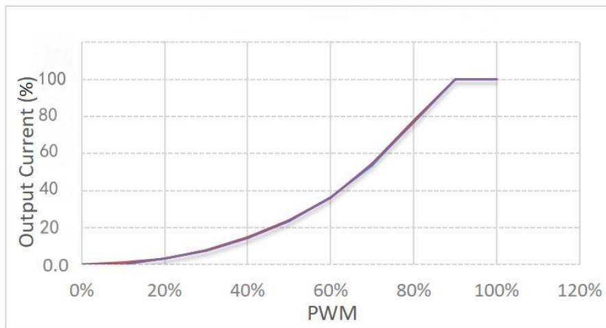
PWM dimming
