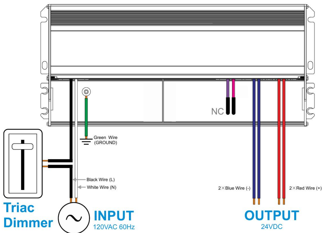
Wiring diagram of 3-in-1 dimming
