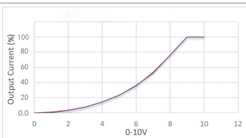
0-10V dimming
