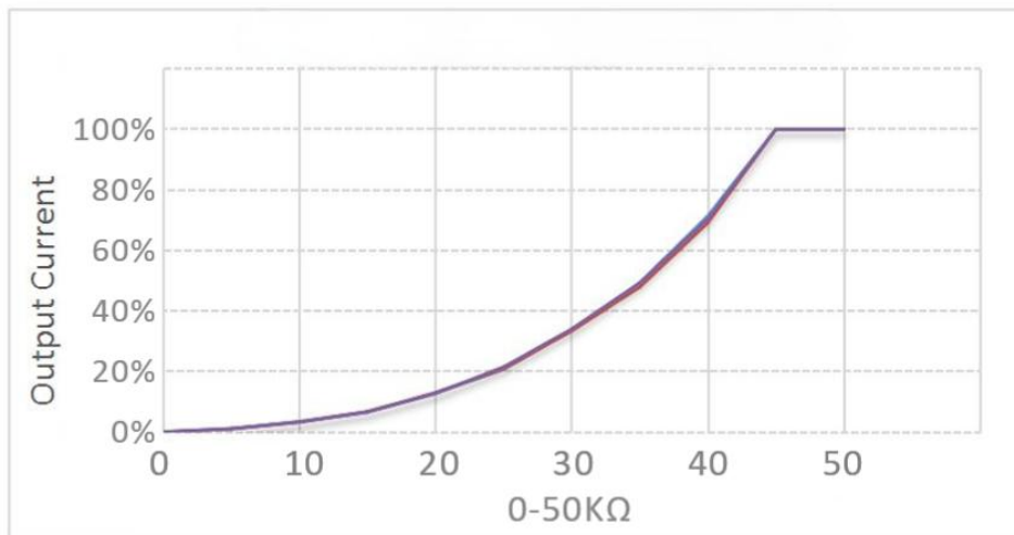
Rx dimming
