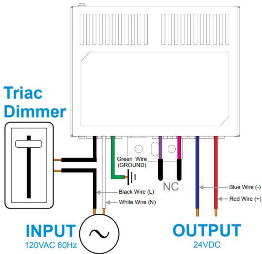
Wiring diagram of Triac dimming
