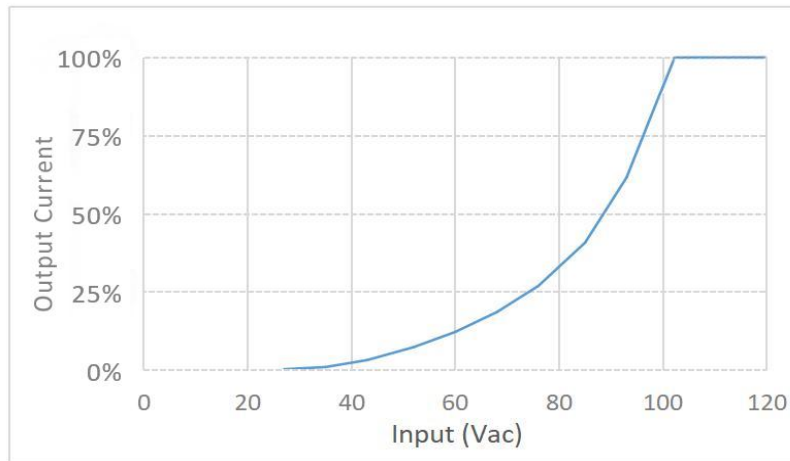
Triac dimming
