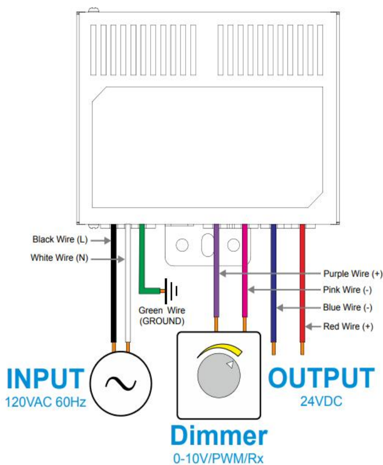
Wiring diagram of 3-in-1 dimming
