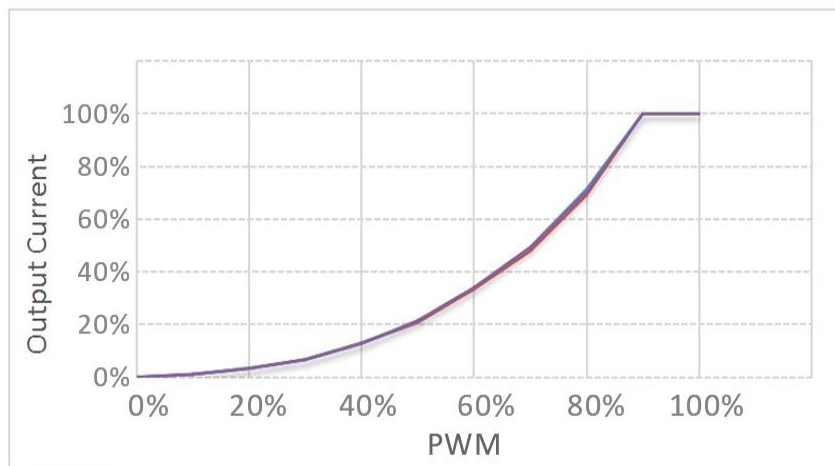
PWM dimming
