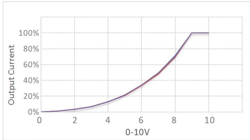
0-10V dimming
