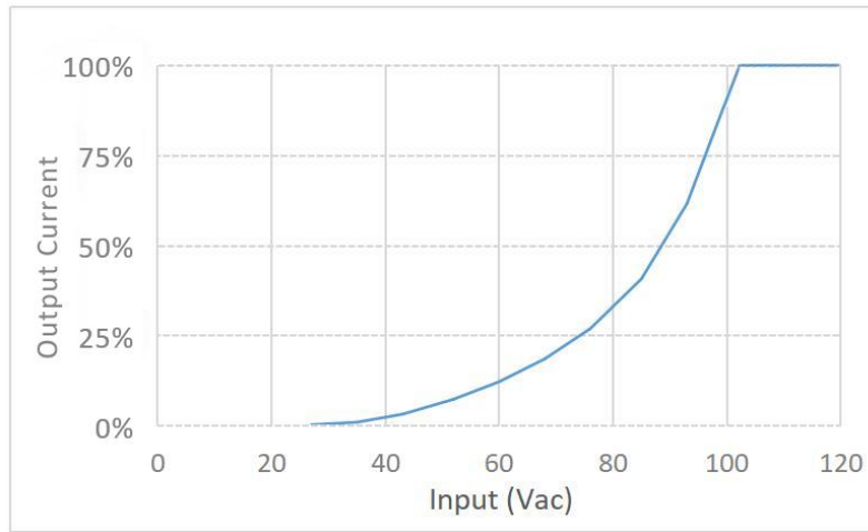
Triac dimming
