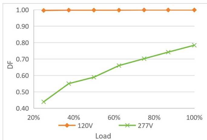
Displacement Factor vs Load
