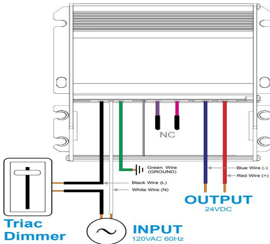
Wiring diagram of Triac dimming
