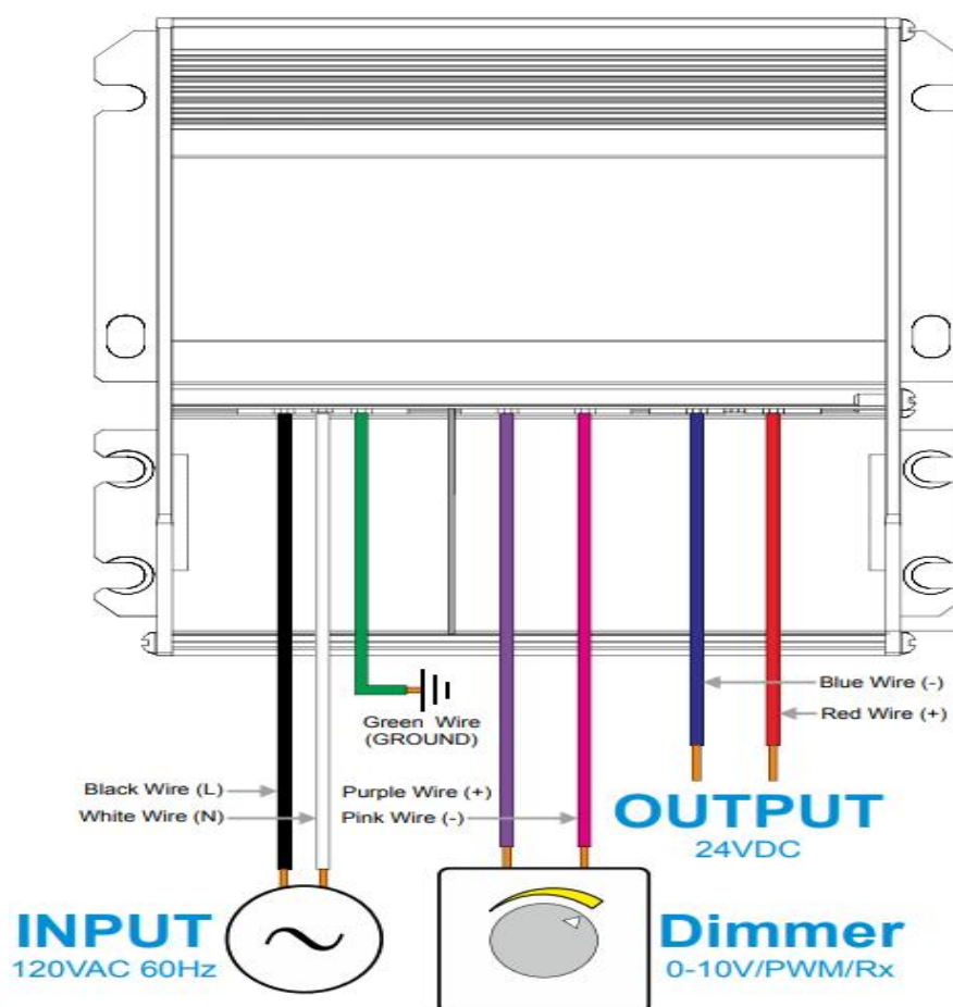
Wiring diagram of 3-in-1 dimming
