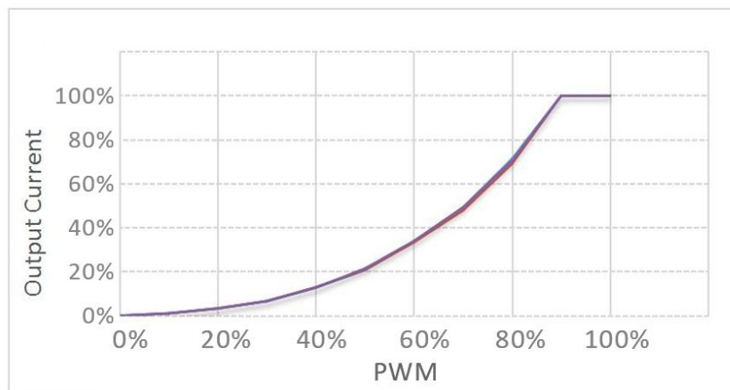
PWM dimming
