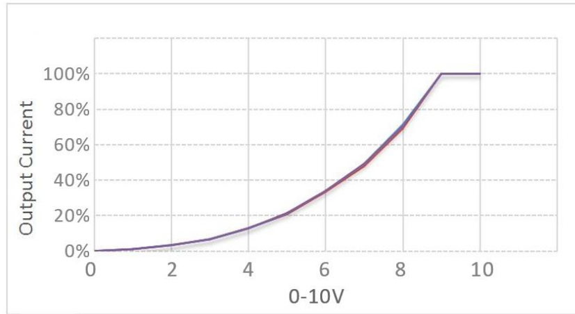
0-10V dimming
