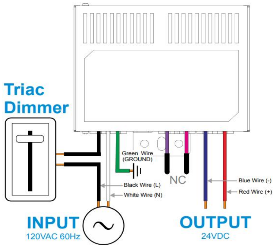
Wiring diagram of Triac dimming
