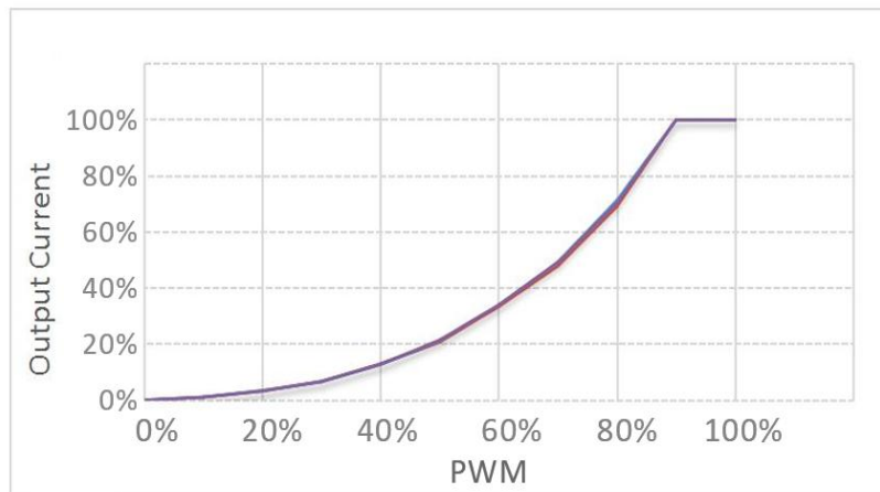
PWM dimming
