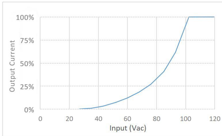
Triac dimming
