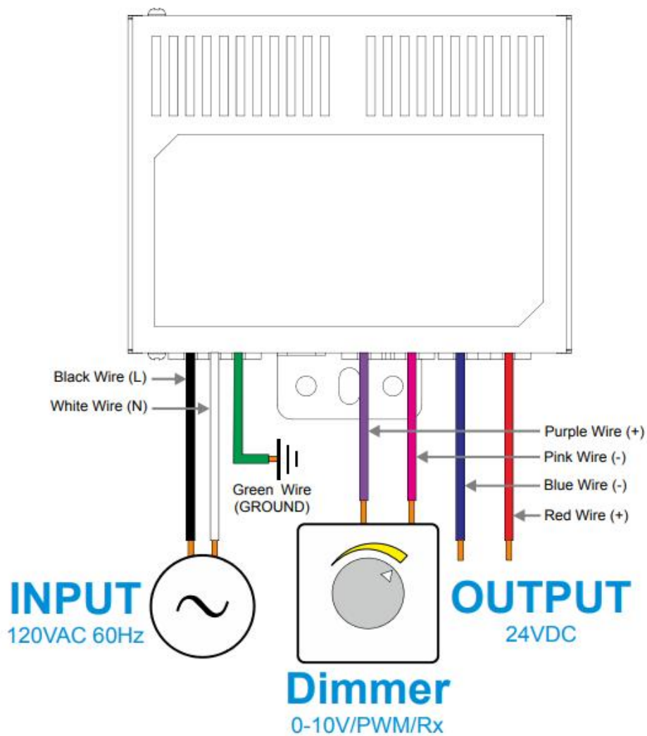
Wiring diagram of 3-in-1 dimming
