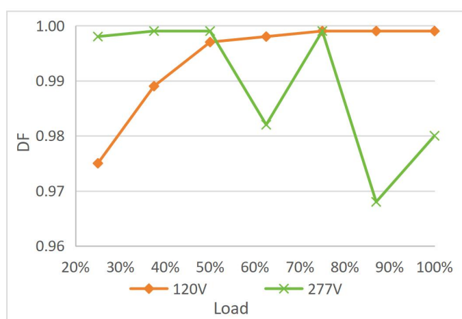
Displacement Factor vs Load
