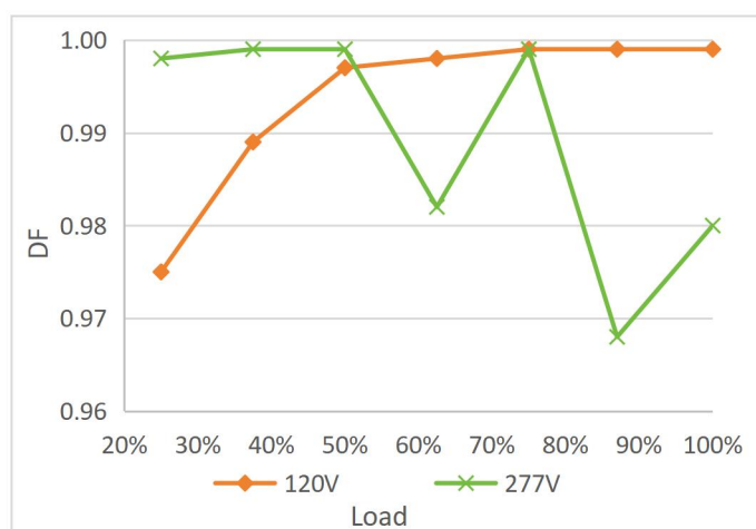
Displacement Factor vs Load
