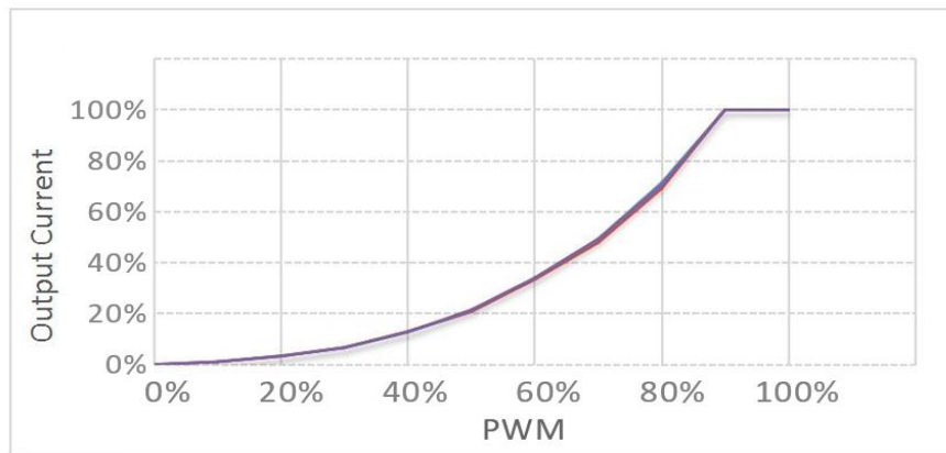
PWM dimming
