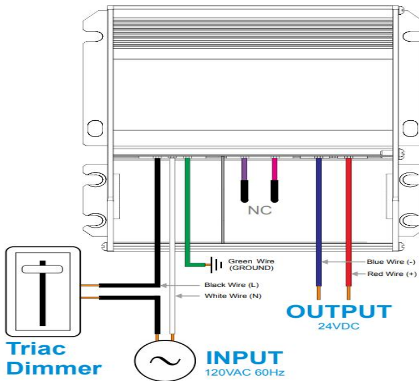
Wiring diagram of Triac dimming
