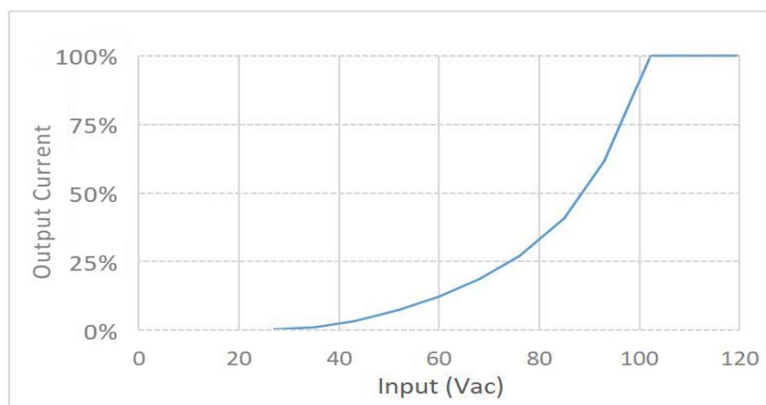
Triac dimming
