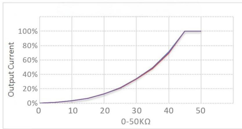
Rx dimming
