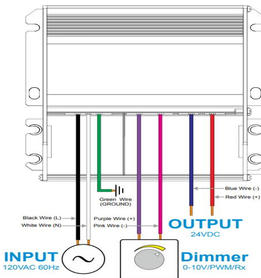
Wiring diagram of 3-in-1 dimming
