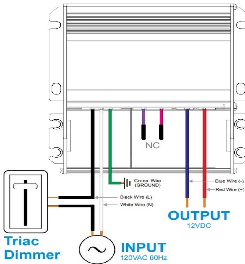
Wiring diagram of Triac dimming
