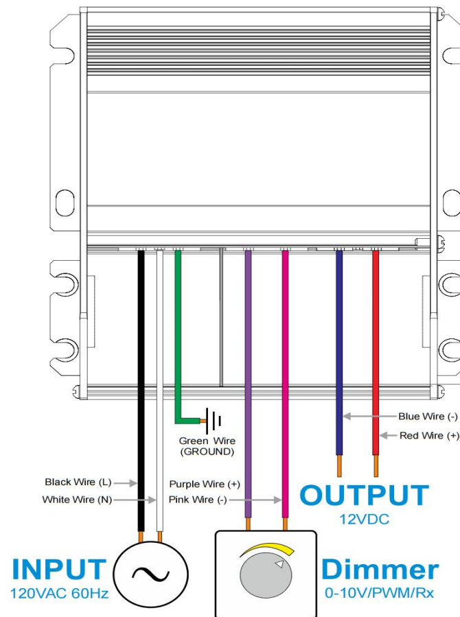
Wiring diagram of 3-in-1 dimming
