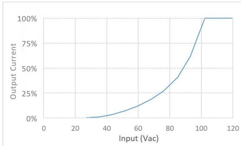
Triac dimming
