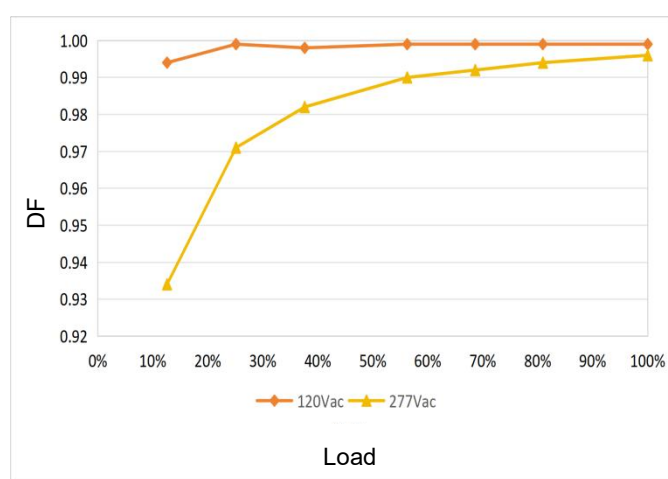
Displacement Factor vs Load
