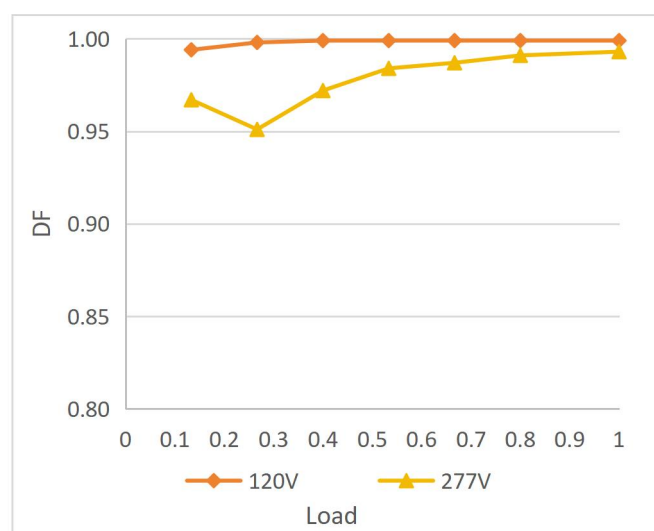
Displacement Factor vs Load
