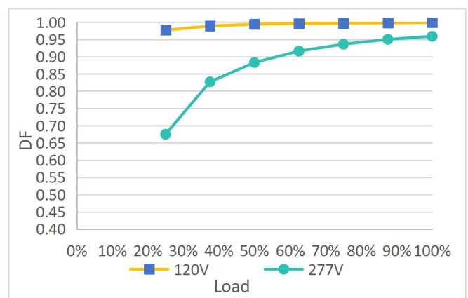
Displacement Factor vs Load
