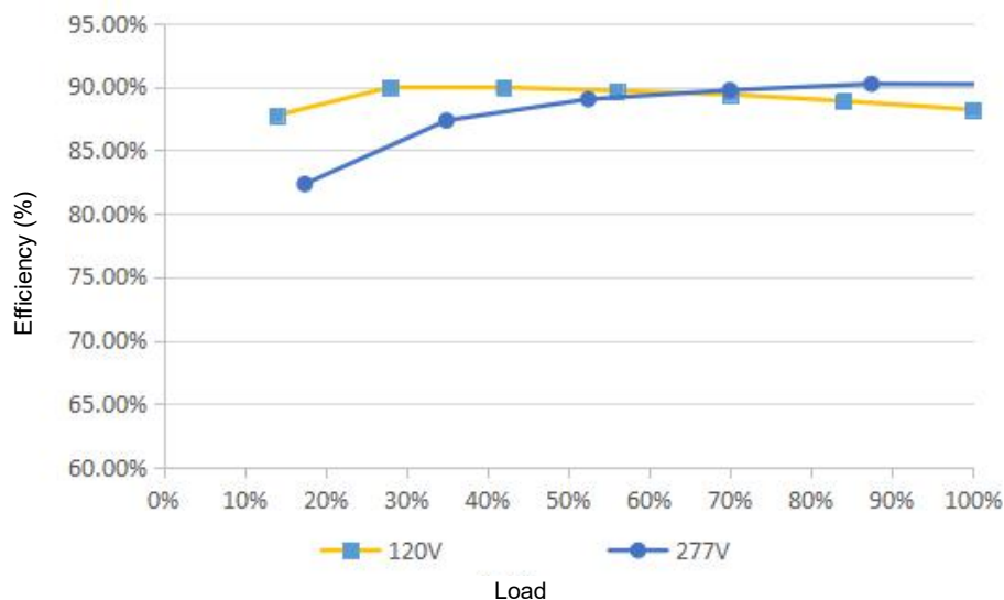
Typical Efficiency vs Load
