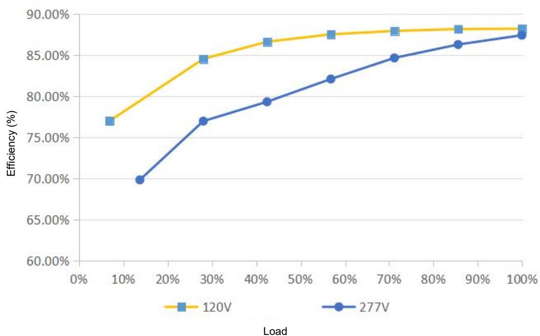
Typical Efficiency vs Load
